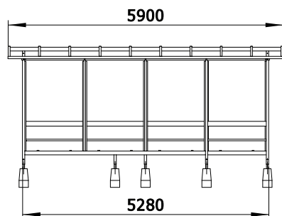
Arret II Duo 207 - 4M
